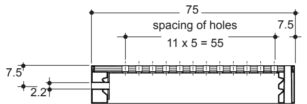
The spacing of the holes of the MP-panels
