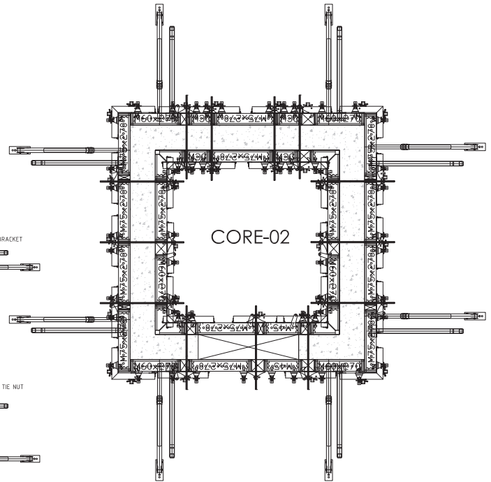
Formwork Layout of Corewall Using Vito Panel
