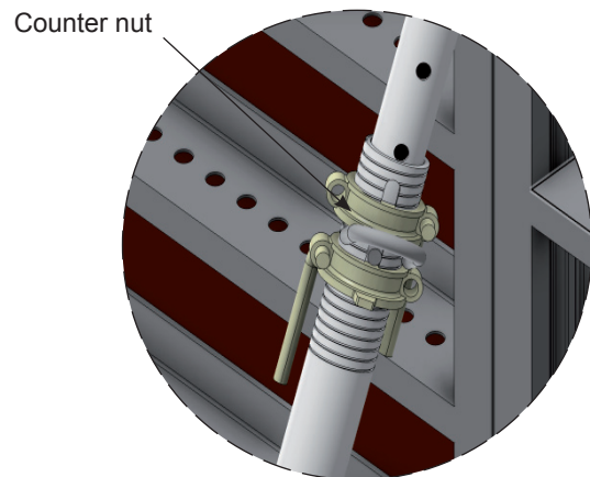
Locking with counter nut
