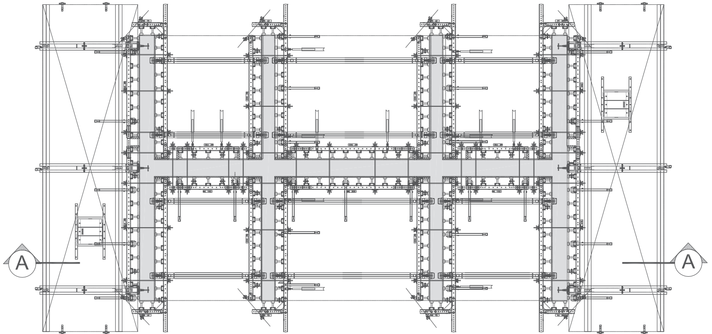
Formwork Layout of Corewall using CBM240
